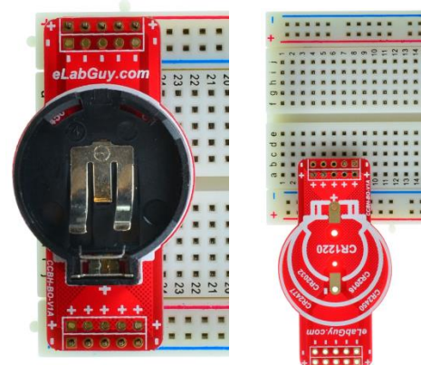
Figure 2: Example of connecting the CR2450-BO-V1A on breadboard
